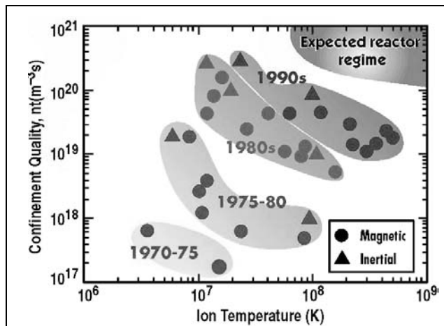
Figure 3 FUSION PROGRESS 1970-2000
