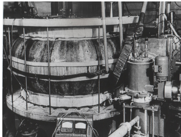
Left: Basic tokamak design. The tokamak features two external magnetic fields (toroidal and poloidal) designed to contain the plasma long enough for fusion reactions to occur. Right: The first tokamak, T-1, in the Soviet Union.
