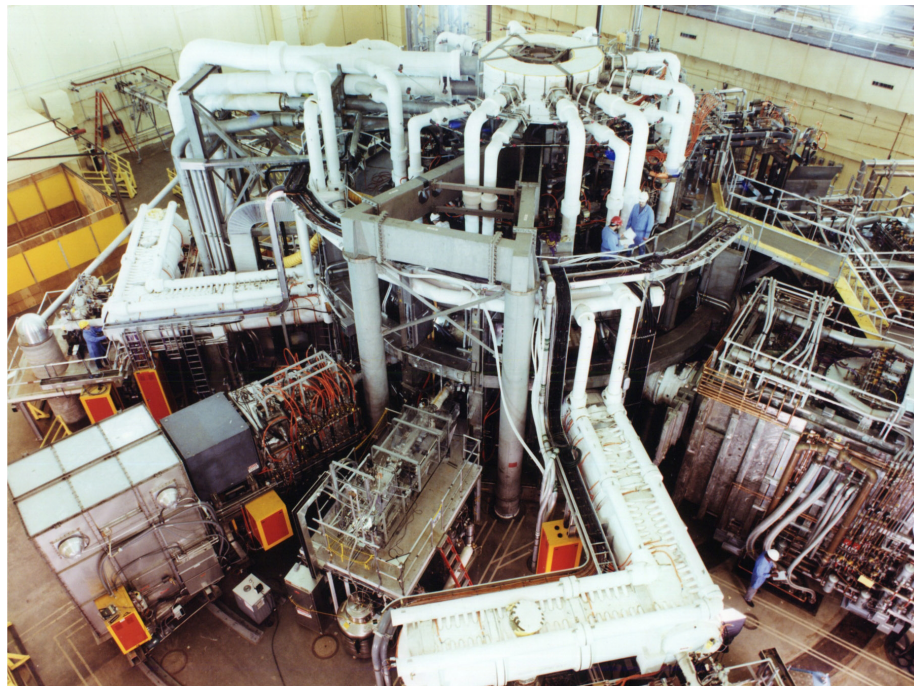
The Tokamak Fusion Test Reactor at Princeton. TFTR operated from 1982 to 1997, setting many significant records both in plasma temperature and in peak fusion power produced, before it was prematurely shut down.
