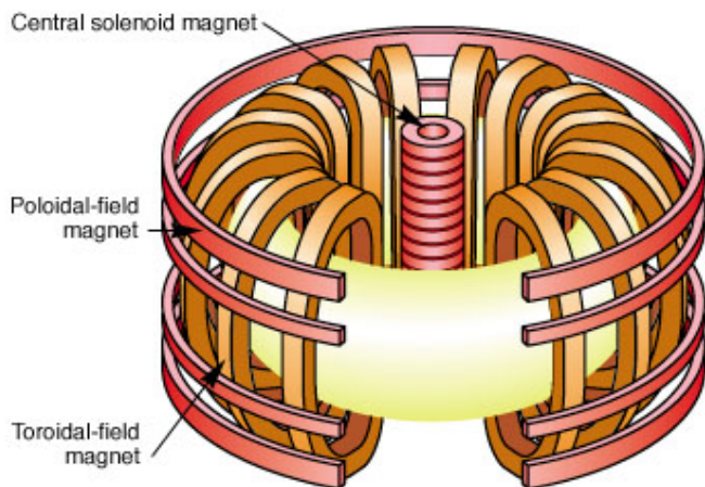
Left: Basic tokamak design. The tokamak features two external magnetic fields (toroidal and poloidal) designed to contain the plasma long enough for fusion reactions to occur. Right: The first tokamak, T-1, in the Soviet Union.
